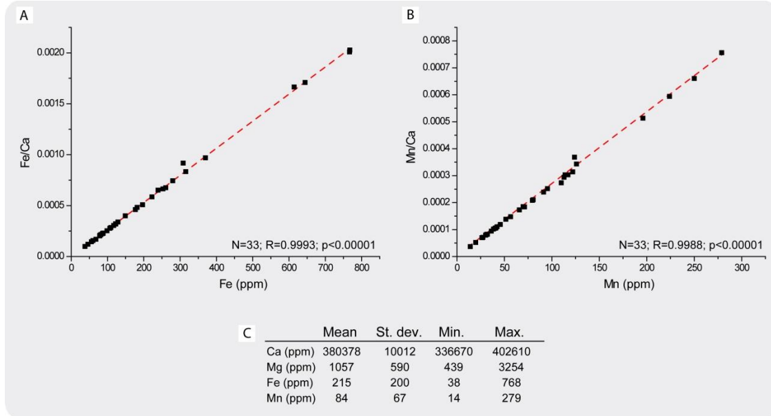
Fig. S3. Comparison between absolute and Ca-corrected values. A and B) Scatter plot and respective linear correlation for absolute values (ppm) and calcium-corrected (element/Ca). Note highly significant correlation ( R>0.99 ) for both Fe and Mn. C) Descriptive statistics (mean, standard deviation, minimum and maximum values) for the elements Ca, Mg, Fe and Mn. Note high mean Ca values even when considering samples that were deliberately sampled to include impurities (diagenetic layers and/or encasing matrix). Magnesium values agree with low-magnesium calcite composition (LMC; Chave et al., 1962).
