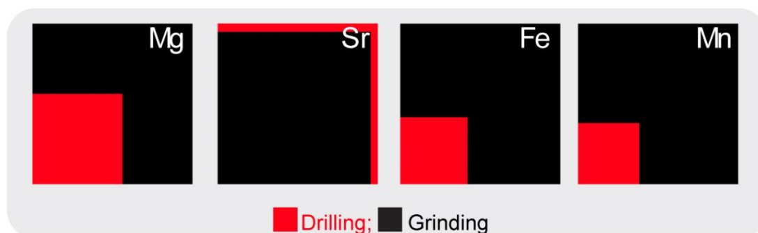
Fig. S4. Proportional differences (larger square equals maximum concentration) between mean elemental concentrations obtained using different sampling protocols (drilling versus grinding). Note a more expressive degree of influence on Fe and Mn elemental abundance obtained via different methods (see main text for details).
