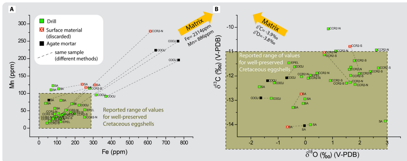
Fig. 3. Geochemical results for all Cretaceous samples used in this study (see also Table 1), including all sample types and tested methods (drilled eggshells, ground eggshells, and encasing matrix). A) Elemental data for Fe plotted against Mn, evident deviation of different sample types follows a clear trend line. B) Isotope crossplot showing most of the samples within the range of expected values, as well as no clear trend lines. Dash line connects results from the same sample; dash rectangle delimits the range of values reported in the literature (Erben et al., 1979; Riera et al., 2013; Eagle et al., 2015; Leuzinger et al., 2021). Abbreviations used for sampled locations according to Fig. S1.
