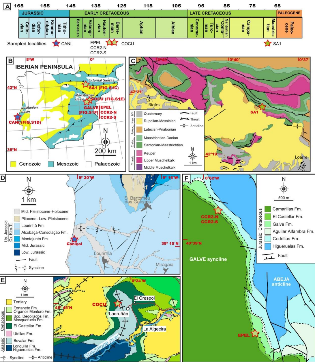
Fig. S1. Fig. S1. Geological setting of the localities from where eggshell samples were collected. A) Chronostratigraphic chart showing the approximate ages of the sampled localities. B) Geological map of the Iberian Peninsula, showing the location of the sampled localities in the Lusitanian Basin, Maestrazgo Basin and External Sierras, with the location of the sampled areas. C) Detailed geological sketch of the External Sierras in the vicinity of Loarre and Riglos municipalities (Huesca, Spain) with the location of Santa Marina 1. D) Detailed geological sketch of the Lusitanian Basin in the vicinity of Lourinhã, showing the location of Caniçal 1 site (Lourinhã, Portugal). E) Detailed geological sketch of
