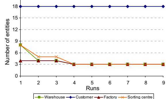
Fig. 20. Network entities.
