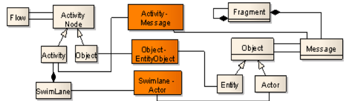
Figure 1 - Activities and Sequence Models Unified Metamodel
