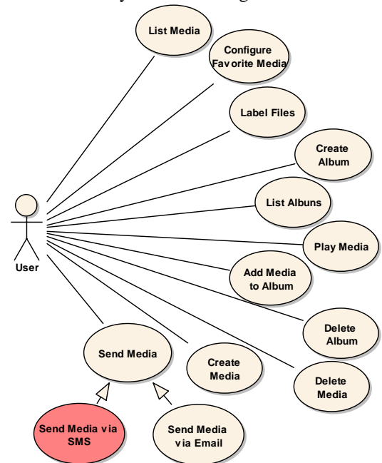
Figure 2 – Use case model for the Mobile Media
