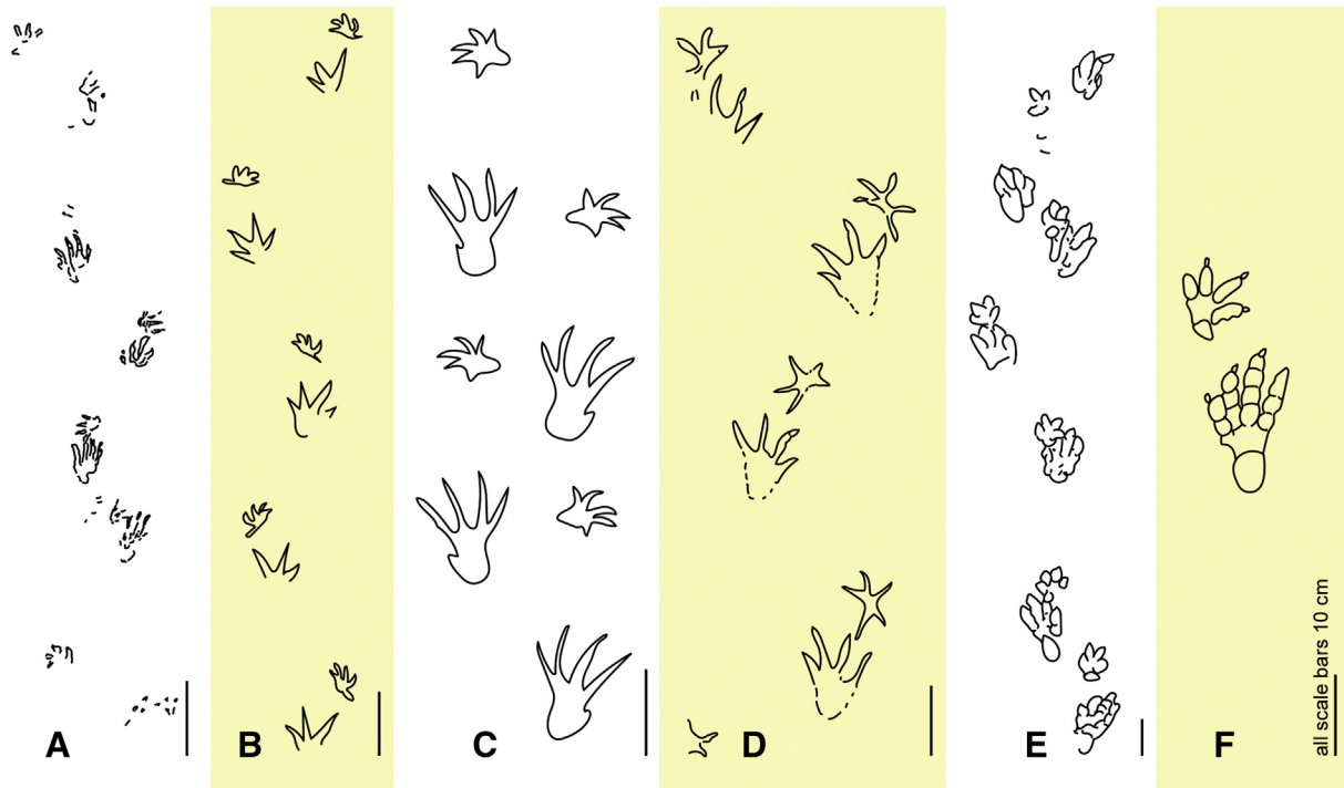
Fig. 9. Interpretative drawings of crocodylomorph trackways. (A) Angolaichnus adamanticus ichnogen. et ichnosp. nov. from the Early Cretaceous of Catoca, Angola; (B) trackway associated to Batrachopus from the Early Jurassic of France; (C) trackway associated to Sustenodactylus from the Early Jurassic of North America; (D) trackway associated to Crocodylopodus from the Jurassic–Cretaceous boundary of Spain; (E) trackway and (F) succession associated to Batrachopus deweyi from the Early Jurassic of North America. B–D after Lockley and Meyer (2004), E and F after Klein and Lucas (2010).
