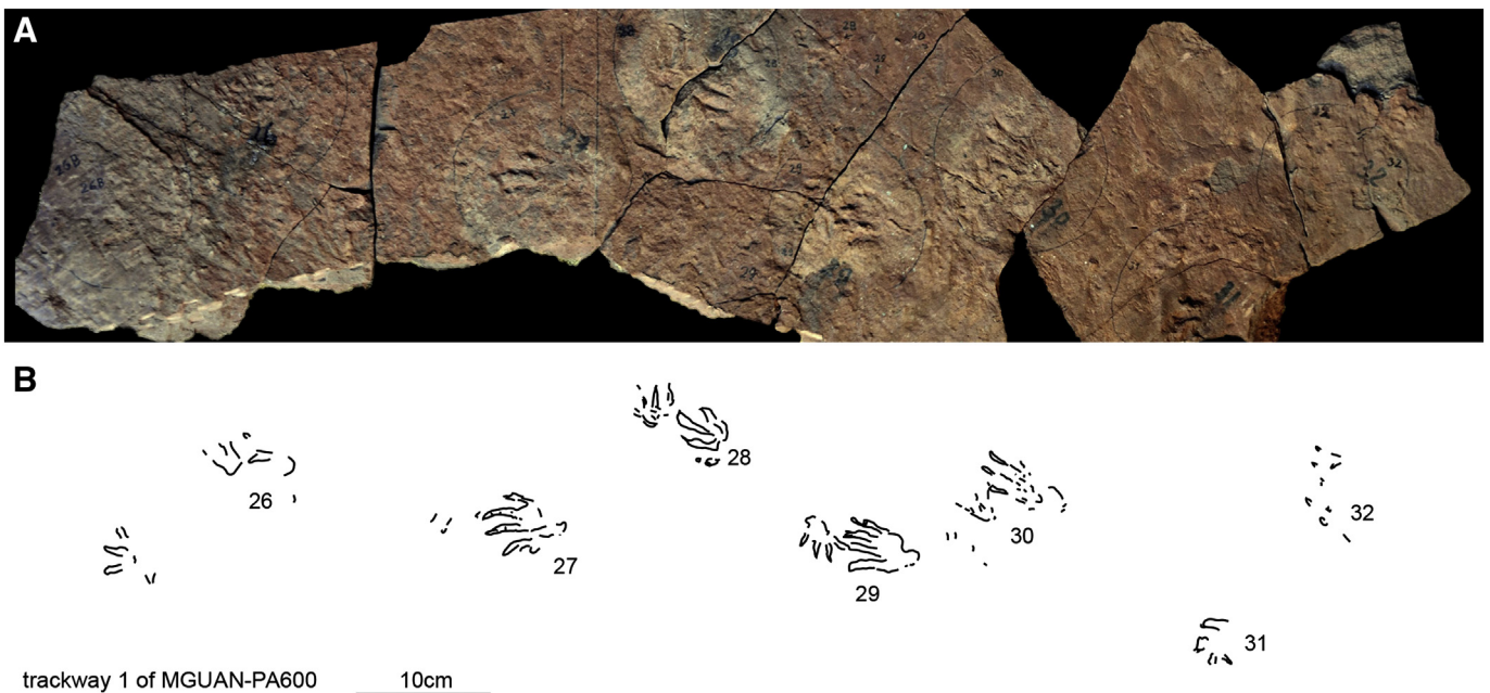
Fig. 4. Angolaichnus adamanticus ichnogen. et ichnosp. nov. holotype trackway 1 in MGUAN-PA600. (A) photograph; (B) interpretative drawing.
