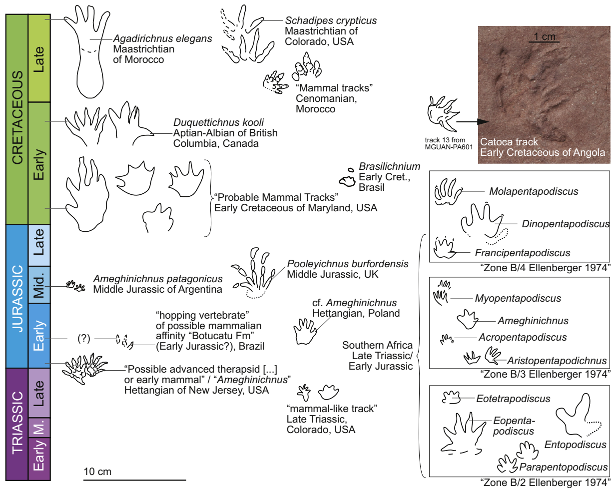
Fig. 8. Mesozoic mammalian track record with Catocapes angolanus ichnogen. et ichnosp. nov. holotype track 13 photograph (right) and interpretative drawing (left).
