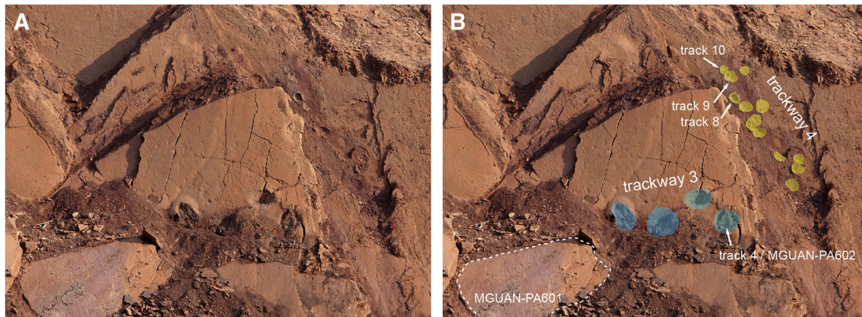
Fig. 5. (A) Overview of the dinosaur trackways from the Catoca mine; (B) annotated version of (A) with the chaotically trampled surface MGUAN-PA601 indicated with the dashed line and sauropod trackway 3 (blue) and sauropod trackway 4 (yellow) with relatively best preserved tracks and the skin impression MGUAN-PA602. (For interpretation of the references to colour in this figure legend, the reader is referred to the web version of this article.)
