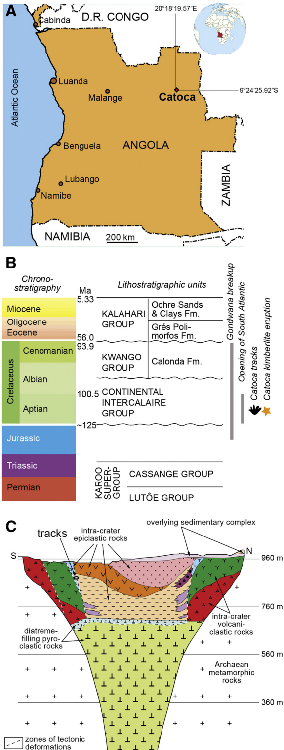
Fig. 1. (A) Catoca global position; (B) Chrono-litho-stratigraphy of “Catoca beds”; (C) Model of the Catoca sedimentary basin (modified after Pervov et al., 2011).
