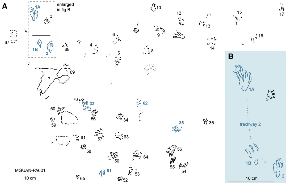
Fig. 3. (A) Drawing based on the field sketch made by OM of the chaotically trampled surfaced bearing mammaliomorph (black) and crocodylomorph (blue) tracks. The broken rectangular line, zoomed in (B), enlightens the possible crocodylomorph trackway 2 and the mammaliomorph track 03. (For interpretation of the references to colour in this figure legend, the reader is referred to the web version of this article.)
