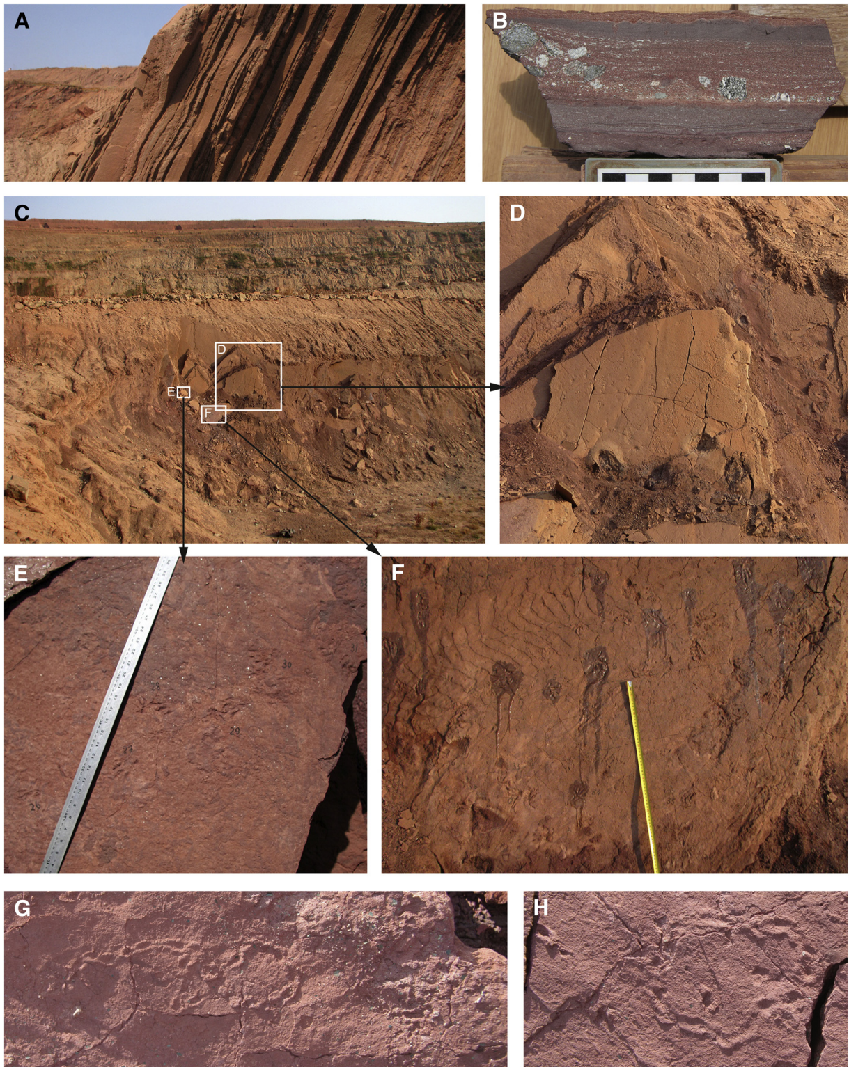
Fig. 2. (A) The sedimentary sequence including footprints of various Mesozoic animals. Intercalation of sand, silt and mudstones. The thickest layer in the center is 15 cm thick. Steep inclination is related to intra-crater tectonic processes; (B) Cross section of a sample with mammal-like animal footprints on its surface. Intercalation of tuffaceous sand-, silt and mudstones. Tuffaceous sandstone includes metamorphic rock clasts and numerous phlogopite flakes. The upper mudstone surface shows desiccation cracks; (C) Overview of the Catoca outcrop in July 2011; photographs in perspective of (D) the two sauropod dinosaur trackway 3 and trackway 4, (E) slab MGUAN-PA600 bearing the crocodylomorph trackway 1, and (F) the chaotically trampled surface MGUAN-PA601 bearing mammaliamorph and crocodylomorph isolated tracks and trackway 2 with evident ripple marks in the upper part; (G) and (H) Scolicia -like snail trails associated with a mud-cracked surface.
