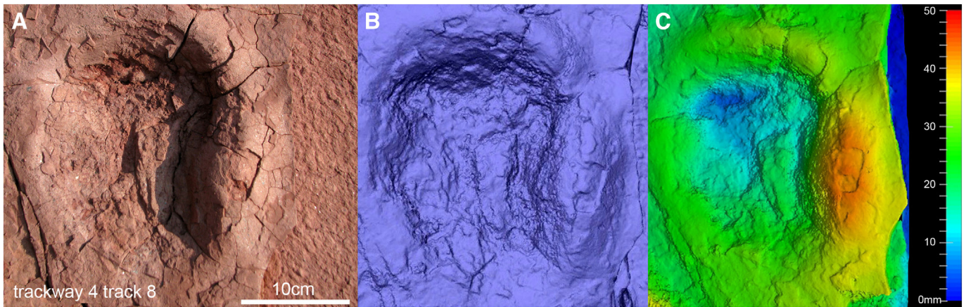
Fig. 10. Sauropod track 8 in trackway 4. (A) photograph; (B) 3D image; (C) photogrammetry derived 3D model in colour-code. (For interpretation of the references to colour in this figure legend, the reader is referred to the web version of this article.)
