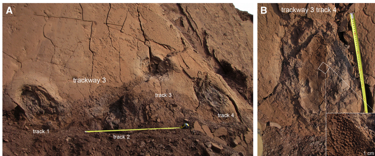
Fig. 6. Sauropod trackway 3. (A) photograph in perspective; (B) photograph of track 4 with the preserved skin impression MGUAN-PA602.
