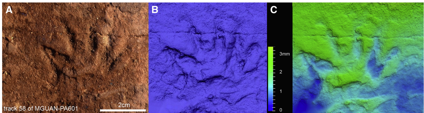
Fig. 12. Catocapes angolanus ichnogen. et ichnosp. nov. paratype track 58 in MGUAN-PA601. (A) photograph; (B) 3D image; (C) photogrammetry derived 3D model in colour-code. (For interpretation of the references to colour in this figure legend, the reader is referred to the web version of this article.)
