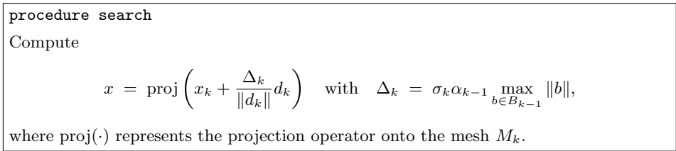
FIG. 7.1. A search step based on the descent indicator.
