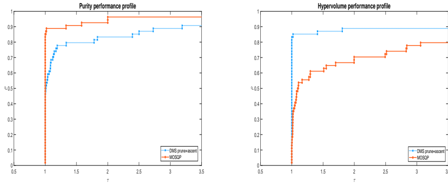
Fig. 5.11: Performance profiles for purity and hypervolume metrics, comparing MOSQP and the new version of DMS, where poll directions are pruned using first order information, but not at all the iterations (1 second of computational time).
