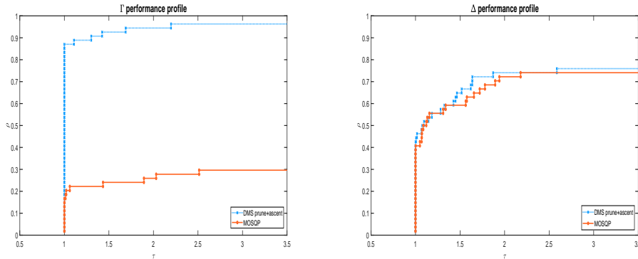
Fig. 5.12: Performance profiles for \Gamma and \Delta metrics, comparing MOSQP and the new version of DMS, where poll directions are pruned using first order information, but not at all the iterations (1 second of computational time).
