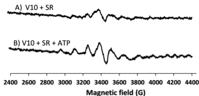
Fig. 4 X-band EPR spectra of 0.5 mM decavanadate (5 mM total vanadate) in 25 mM HEPES (pH 7.0), 100 mM KCl, 5 mM MgCl_2 , 50 \mu\text{M} CaCl_2 with SR calcium ATPase, in the absence (A) and in the presence of 0.25 mM ATP (B). The spectra were acquired as described under Materials and methods. Upon protein addition the oxidovanadium(iv) typical signals are elicited.
